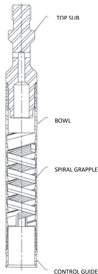
SPIRAL GRAPPLE ASSEMBLY
