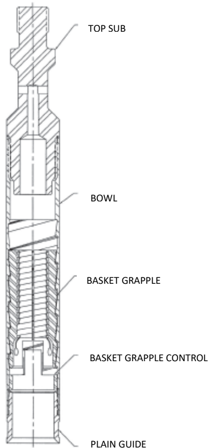
BASKET GRAPPLE ASSEMBLY
